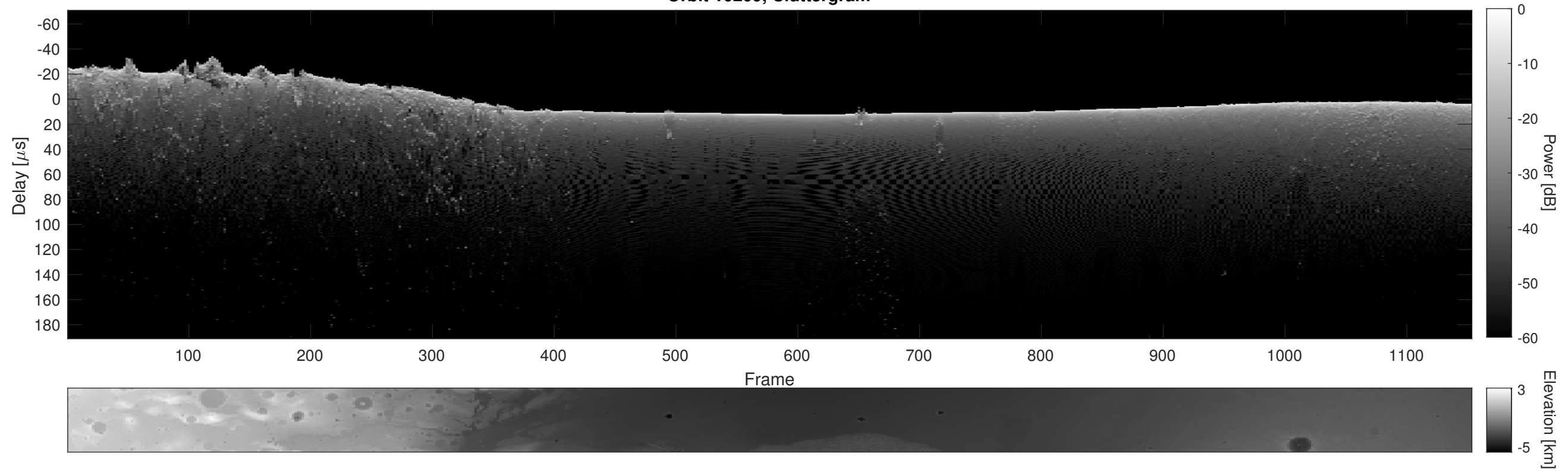
Orbit 10209, Cluttergram
