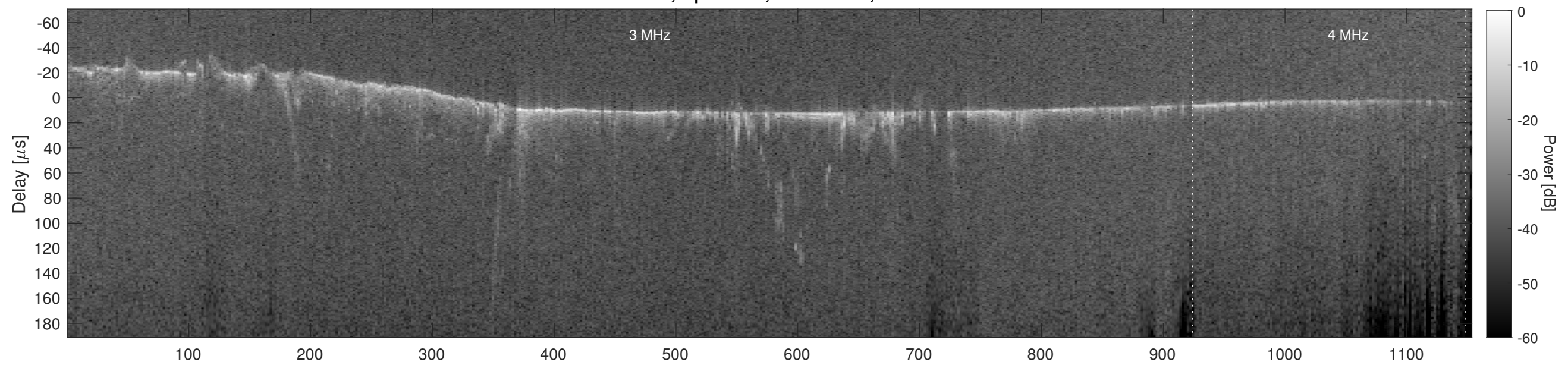
Orbit 10209, Cluttergram
