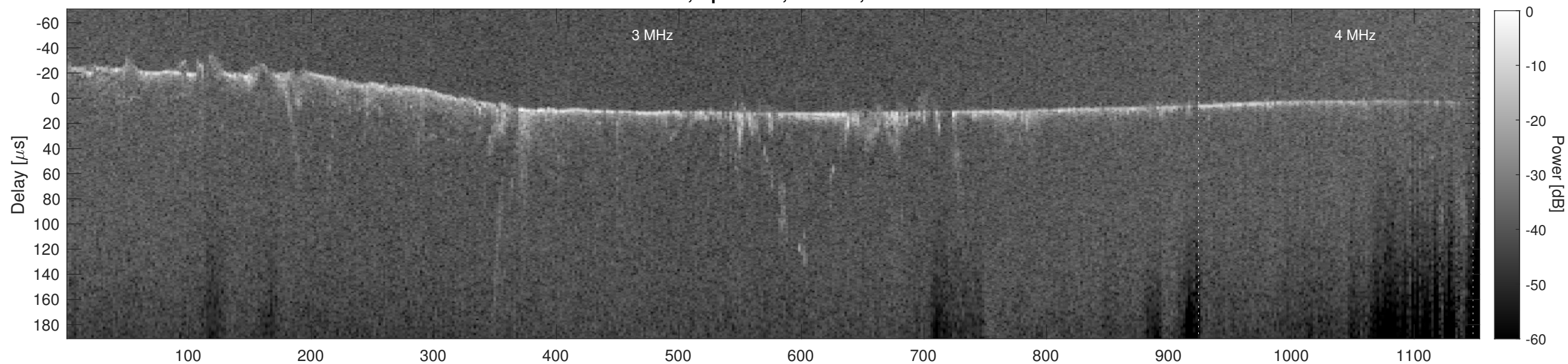
Orbit 10209, Cluttergram
