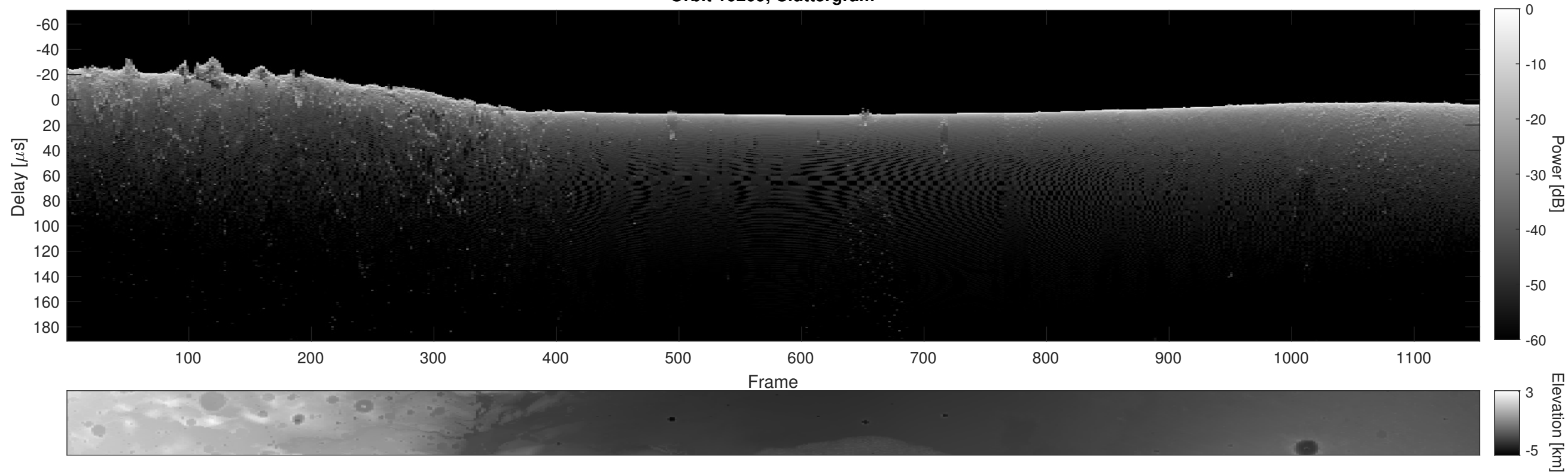
Orbit 10209, Cluttergram
