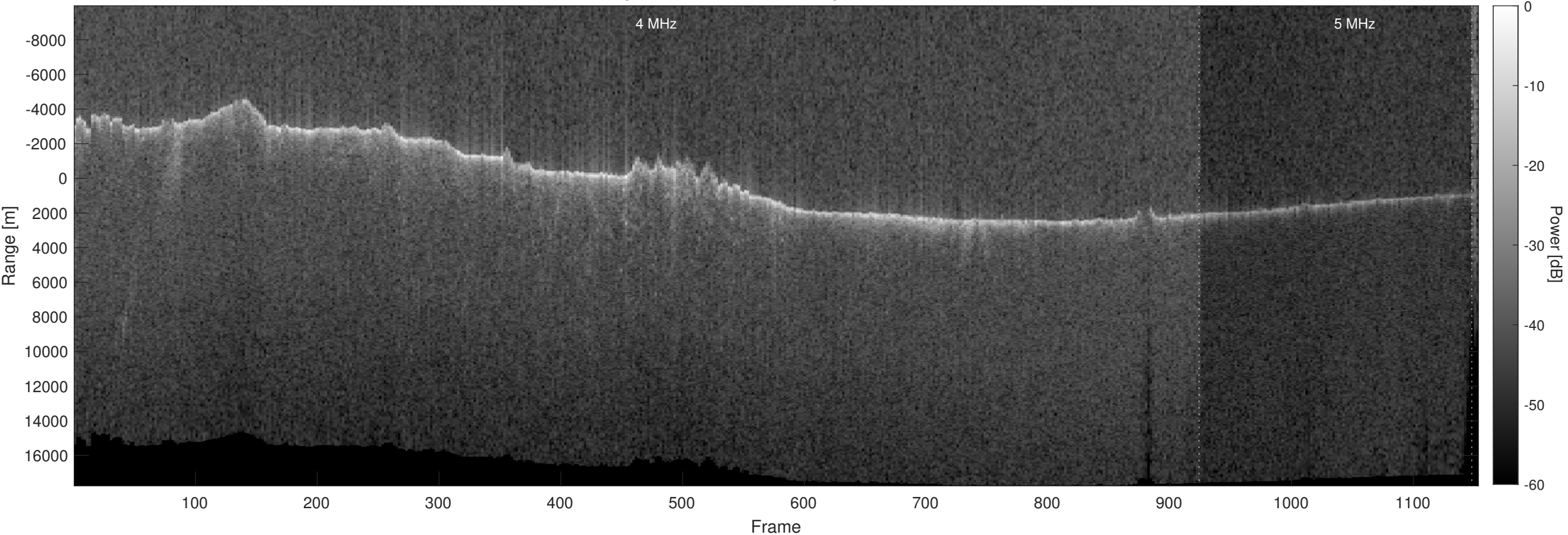
Orbit 10210, Optimized, No Window, Depth-Corrected, Channel 2
