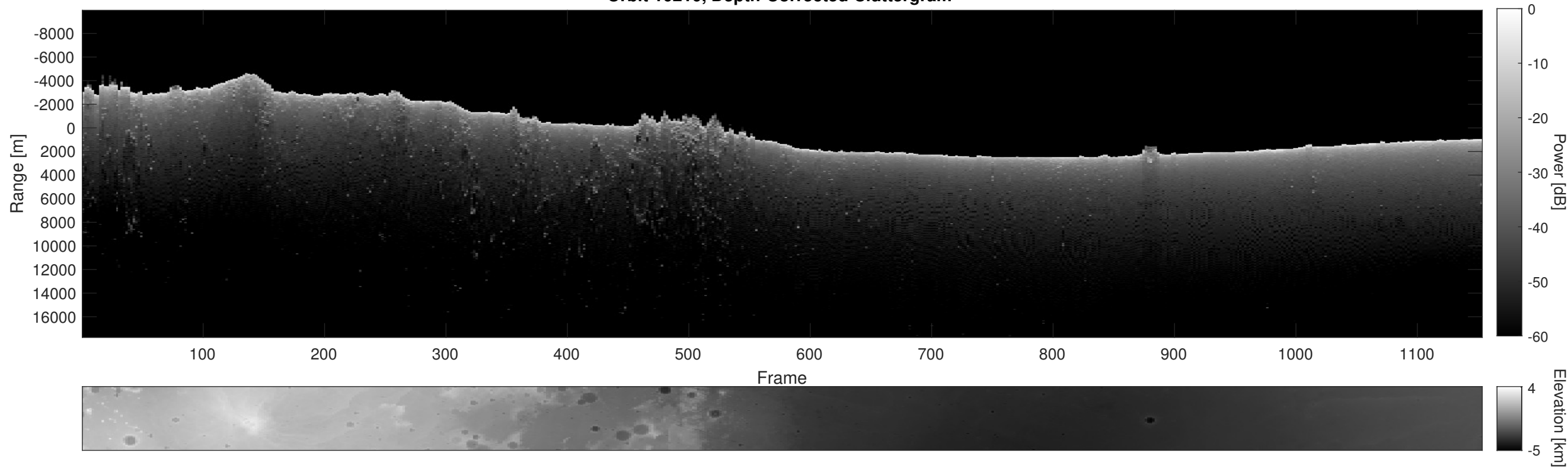
Orbit 10210, Depth-Corrected Cluttergram
