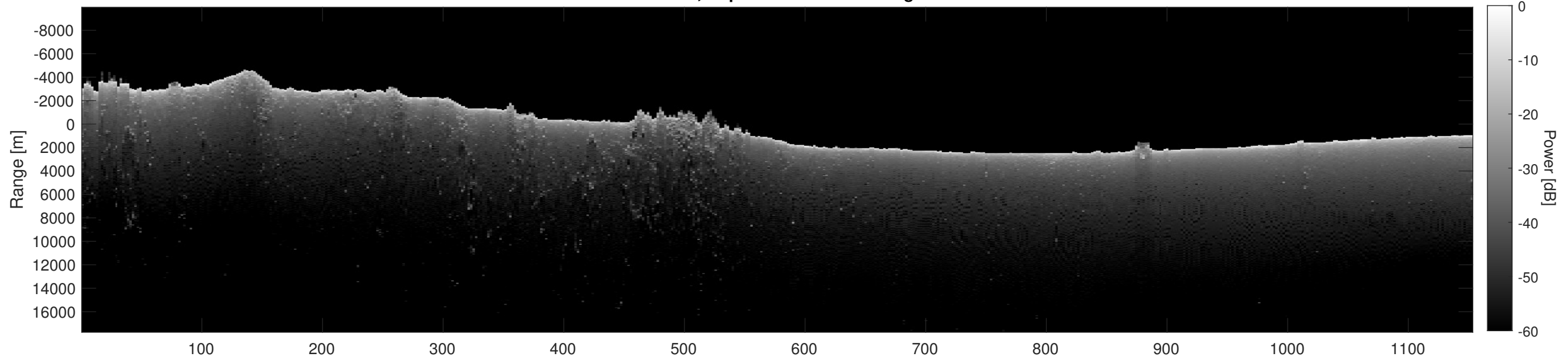
Orbit 10210, Depth-Corrected Cluttergram
