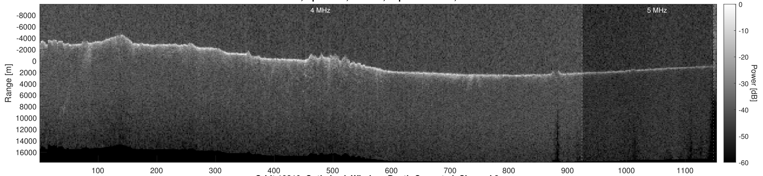
Orbit 10210, Optimized, Window, Depth-Corrected, Channel 2
