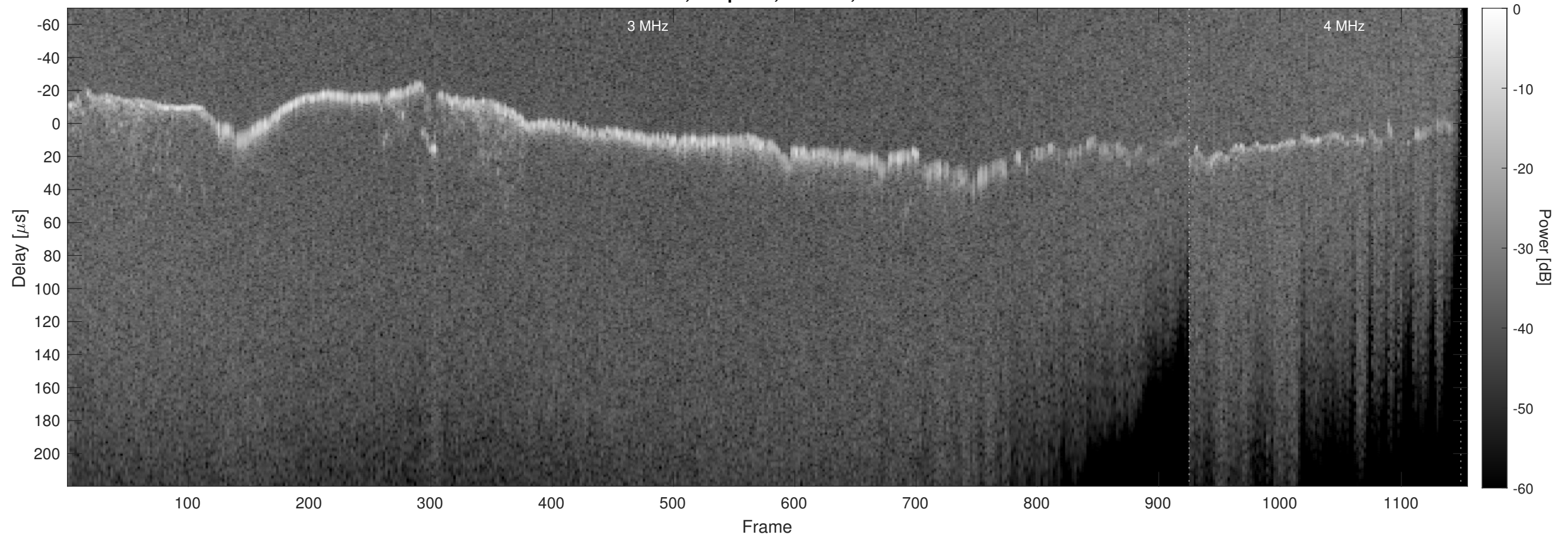
Orbit 10212, Chapman, Window, Channel 2
