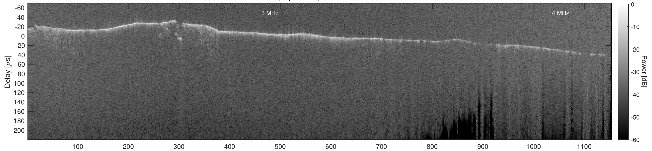
Orbit 10212, Cluttergram
