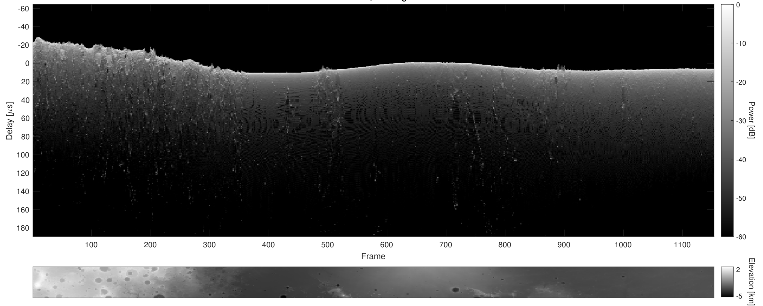
Orbit 10213, Cluttergram
