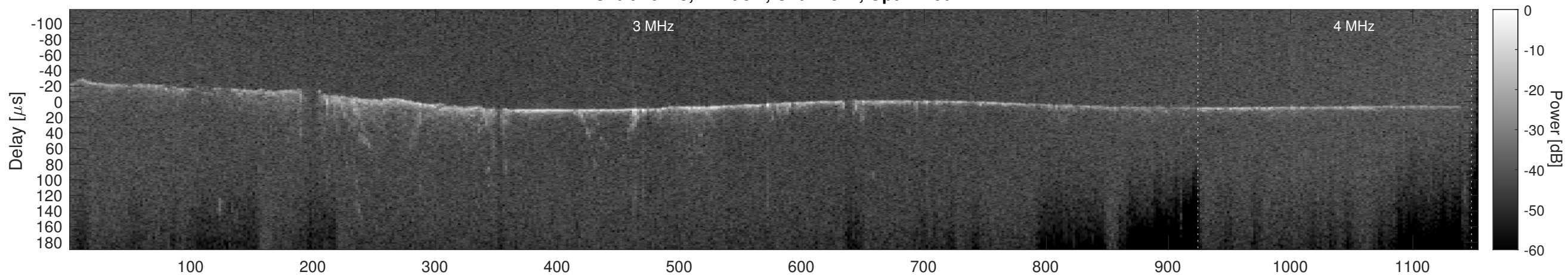
Orbit 10213, Cluttergram
