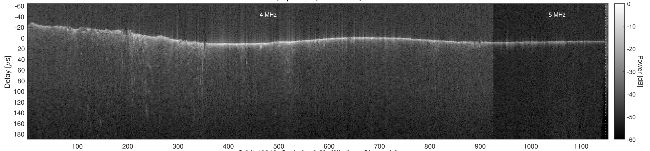
Orbit 10213, Optimized, No Window, Channel 2
