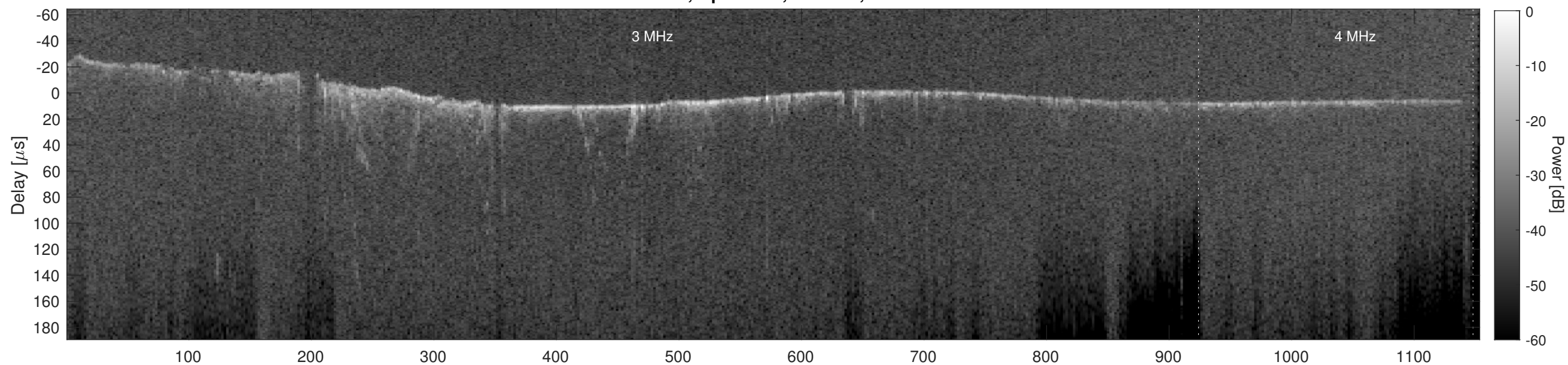
Orbit 10213, Cluttergram
