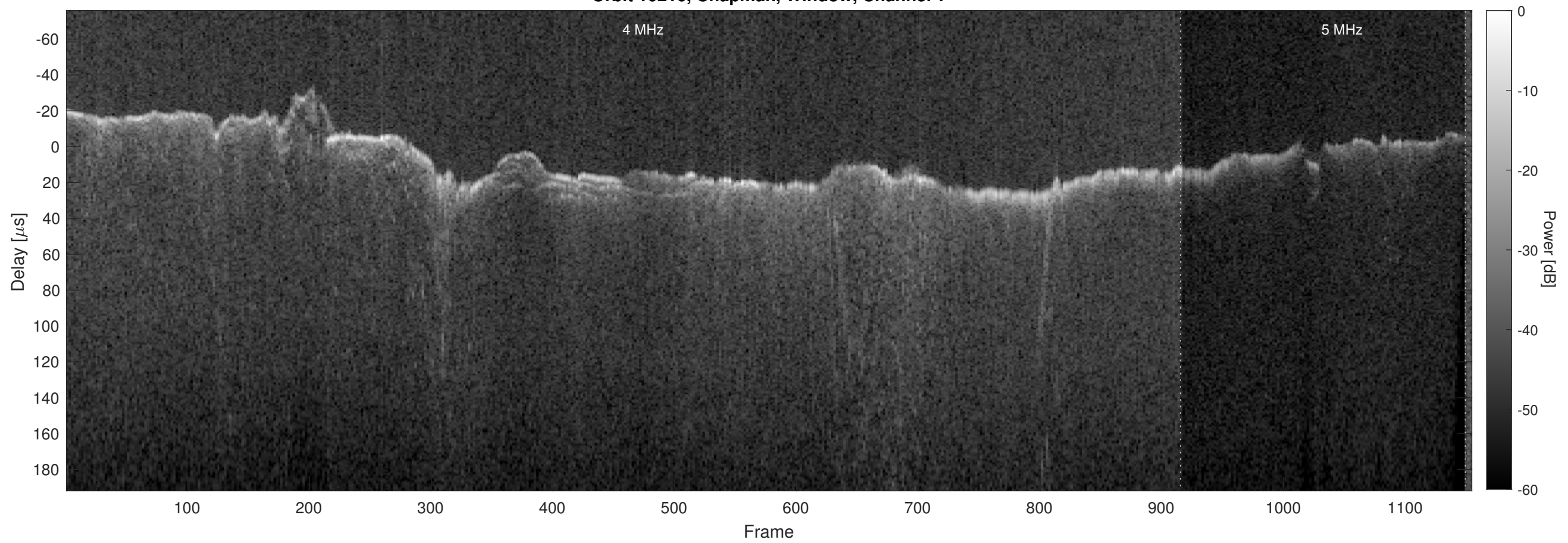
Orbit 10216, Chapman, Window, Channel 2
