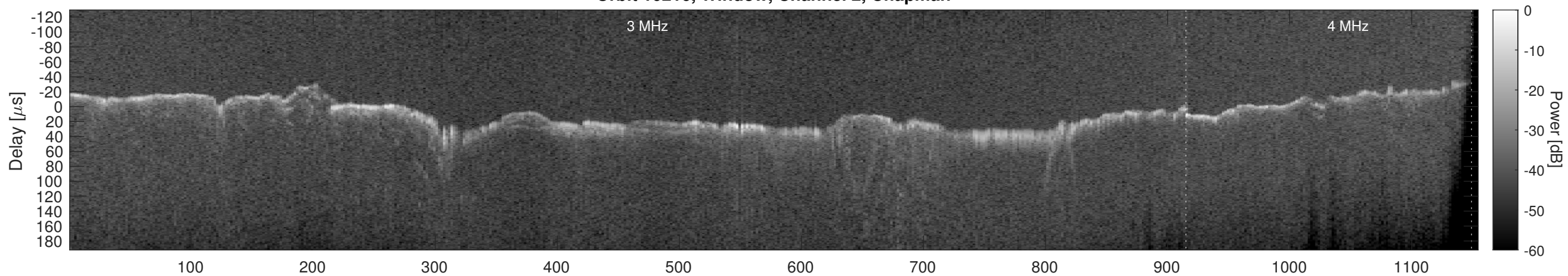
Orbit 10216, Window, Channel 2, Optimized
