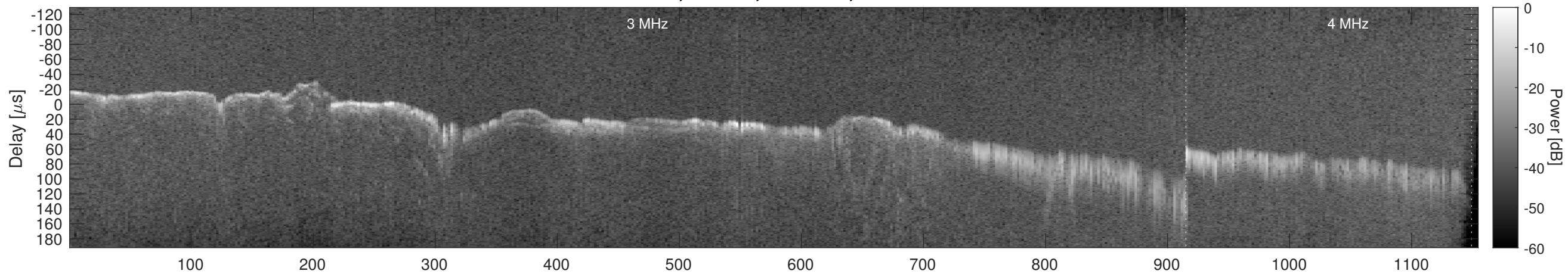
Orbit 10216, Window, Channel 2, Chapman
