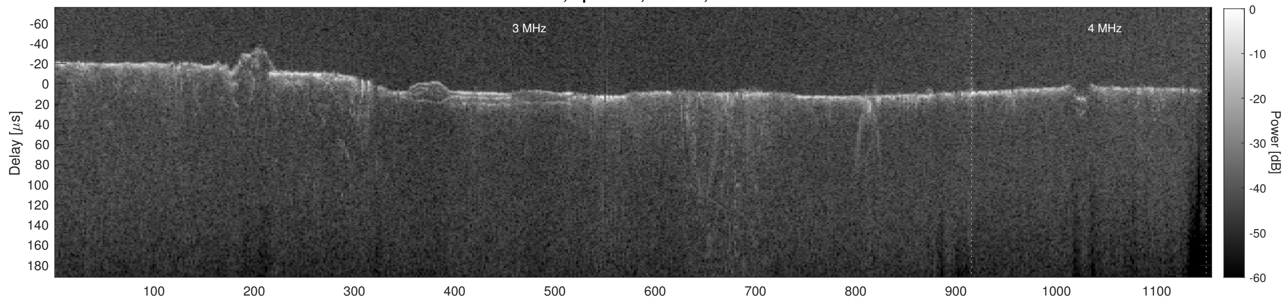
Orbit 10216, Cluttergram
