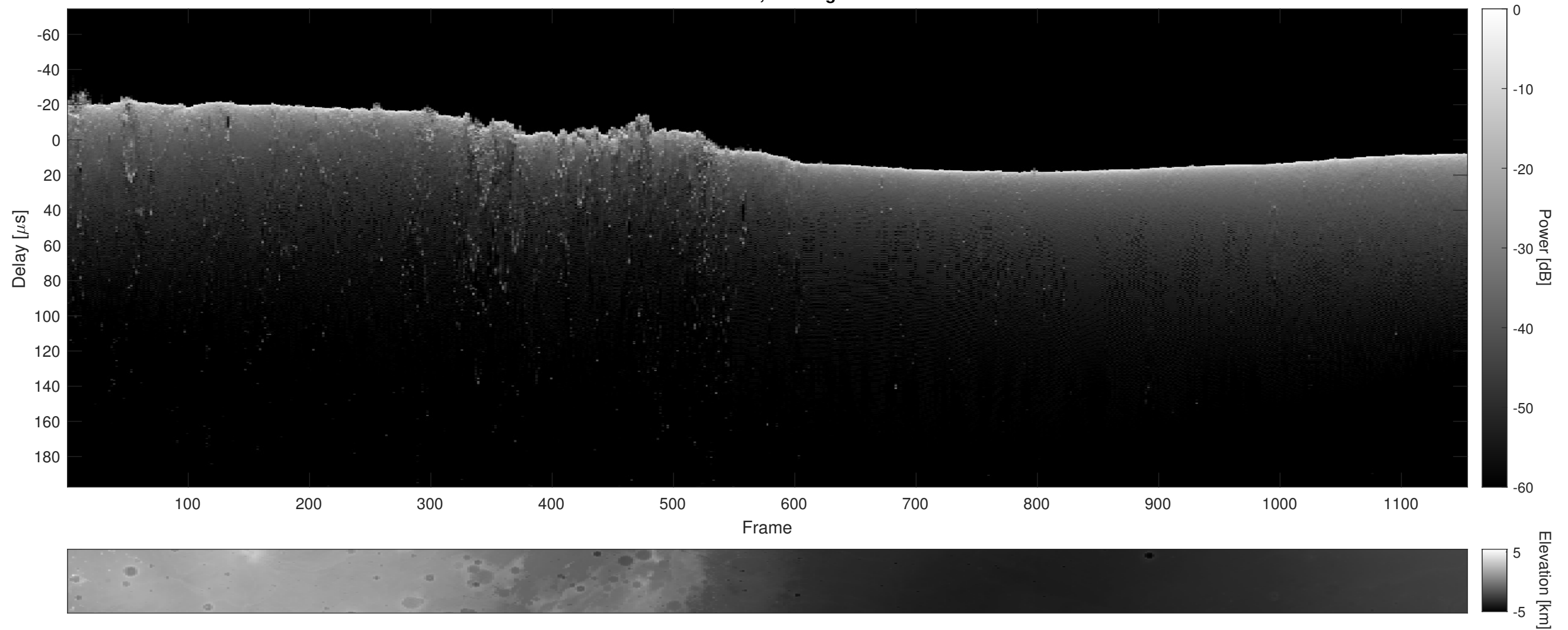
Orbit 10217, Cluttergram
