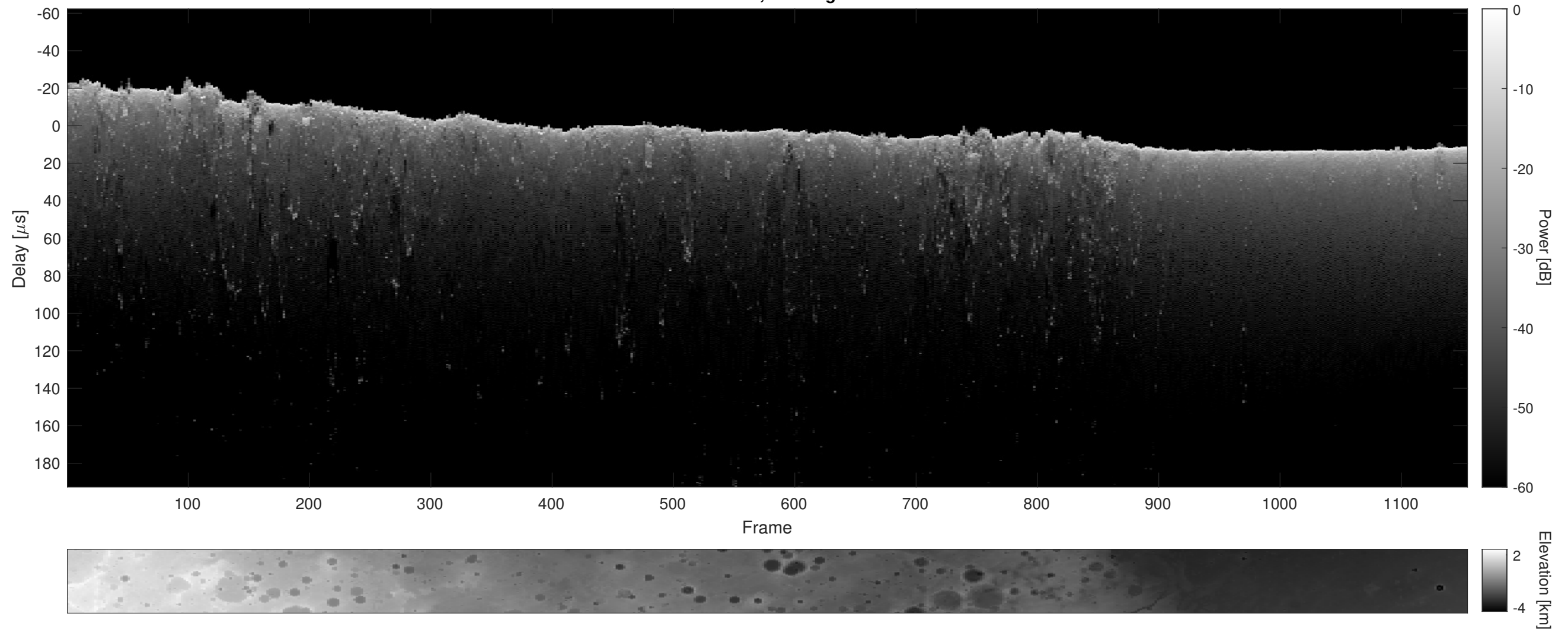
Orbit 10218, Cluttergram
