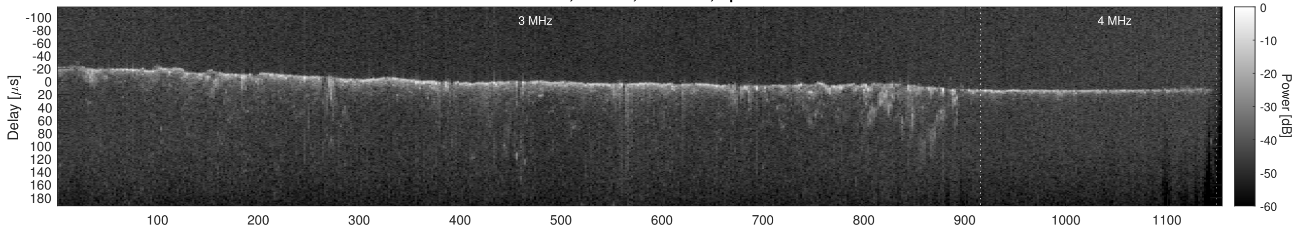
Orbit 10218, Cluttergram
