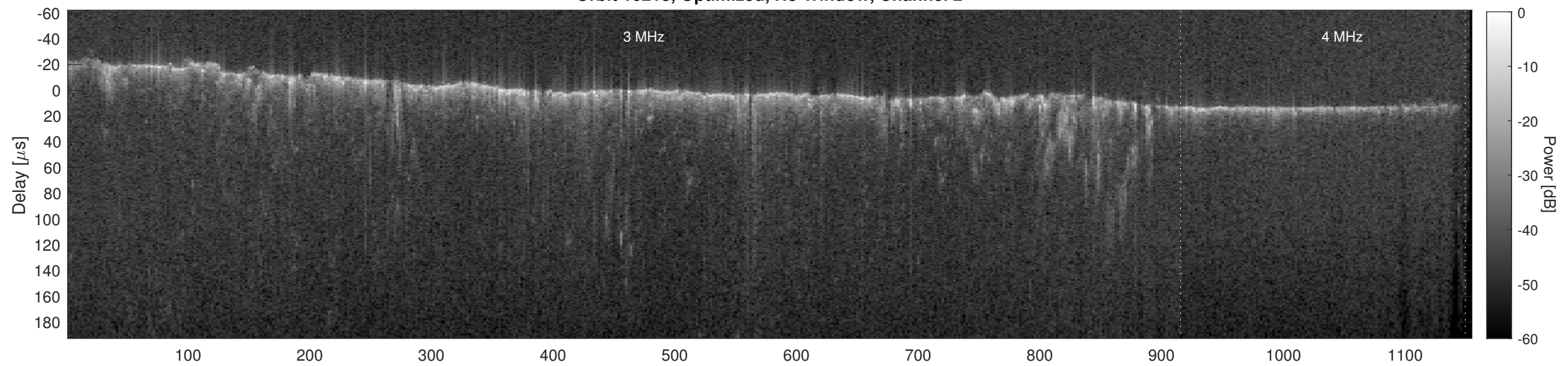
Orbit 10218, Cluttergram
