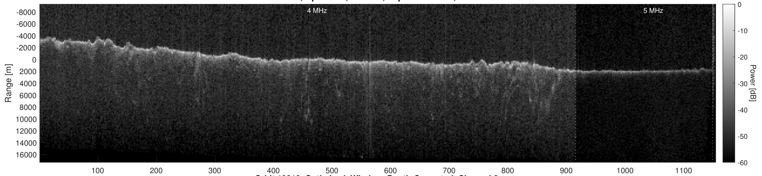
Orbit 10218, Optimized, Window, Depth-Corrected, Channel 2
