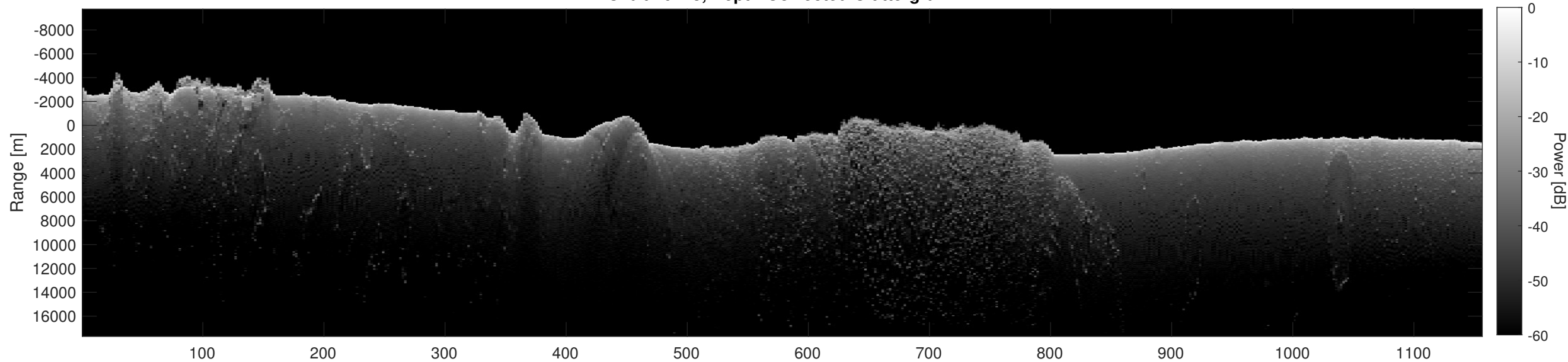
Orbit 10223, Depth-Corrected Cluttergram
