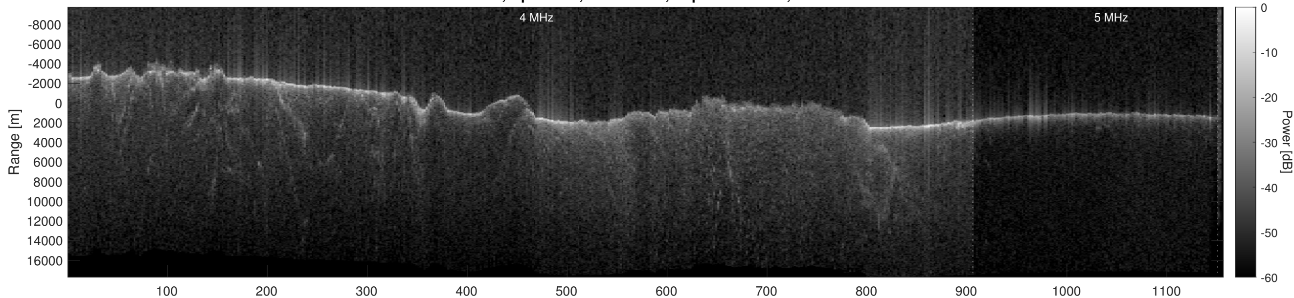
Orbit 10223, Optimized, No Window, Depth-Corrected, Channel 2
