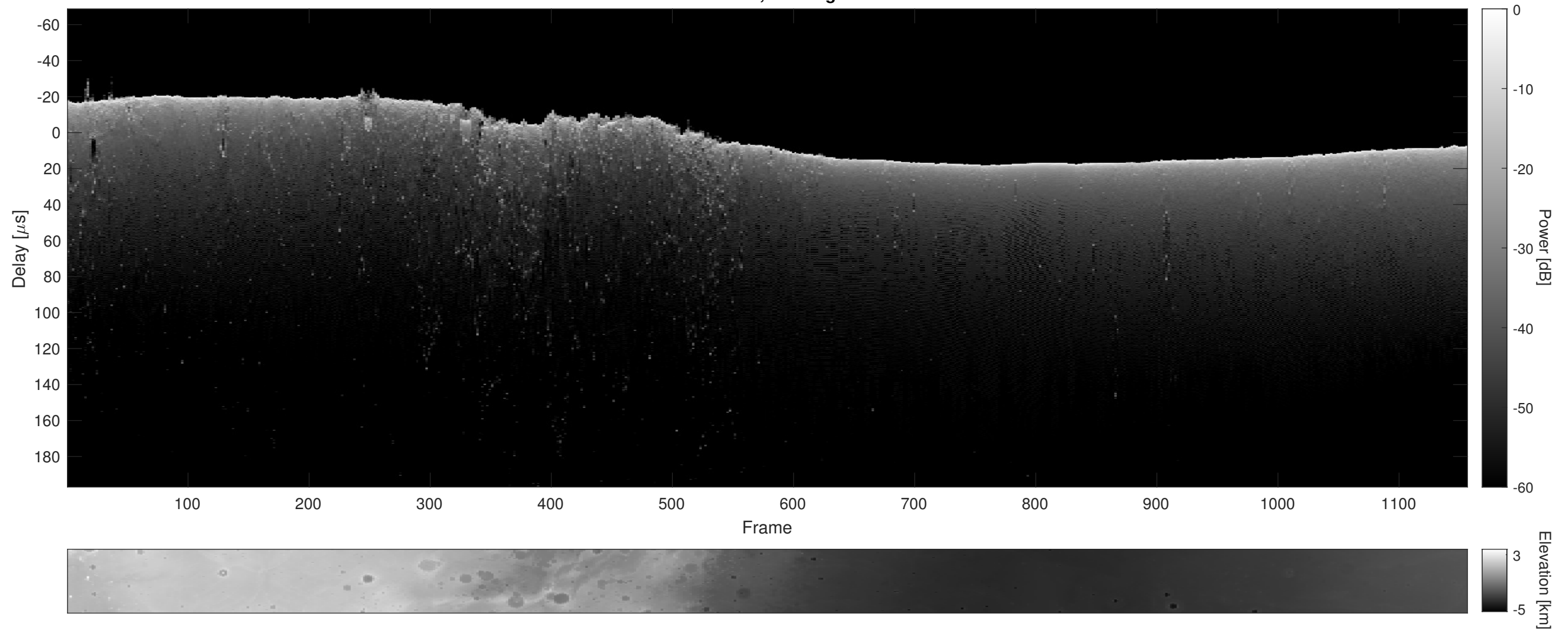
Orbit 10224, Cluttergram
