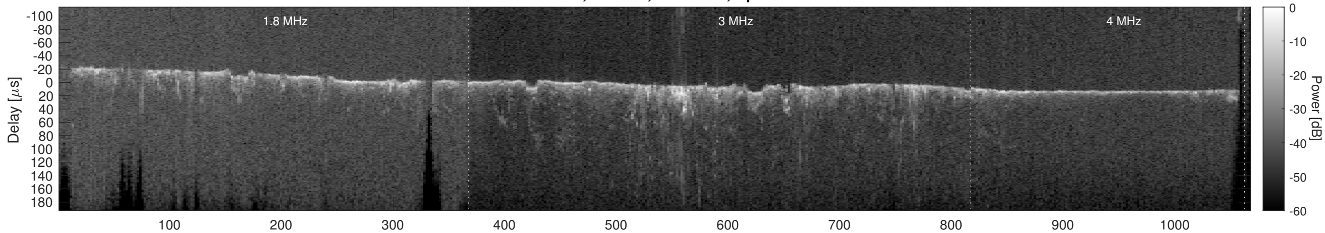
Orbit 10225, Cluttergram
