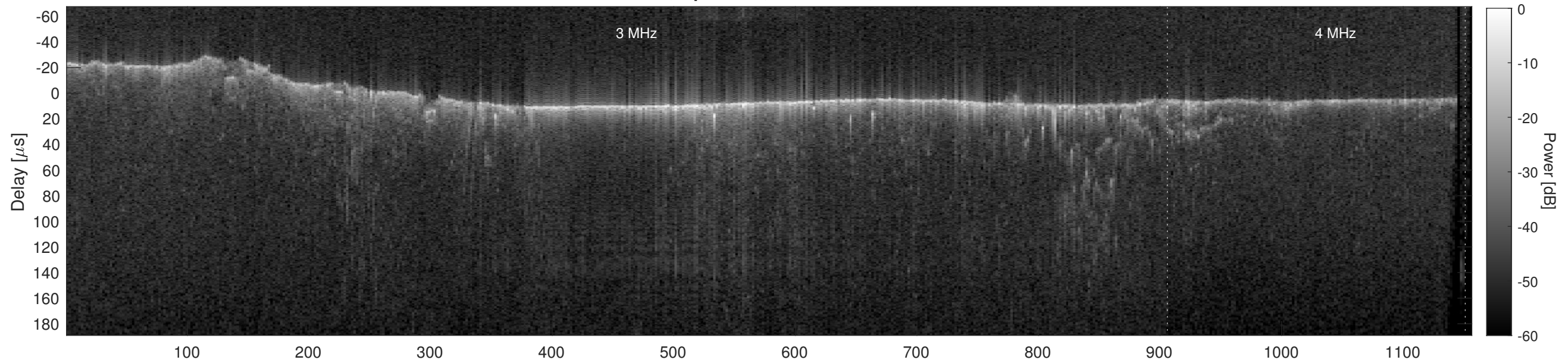
Orbit 10227, Cluttergram
