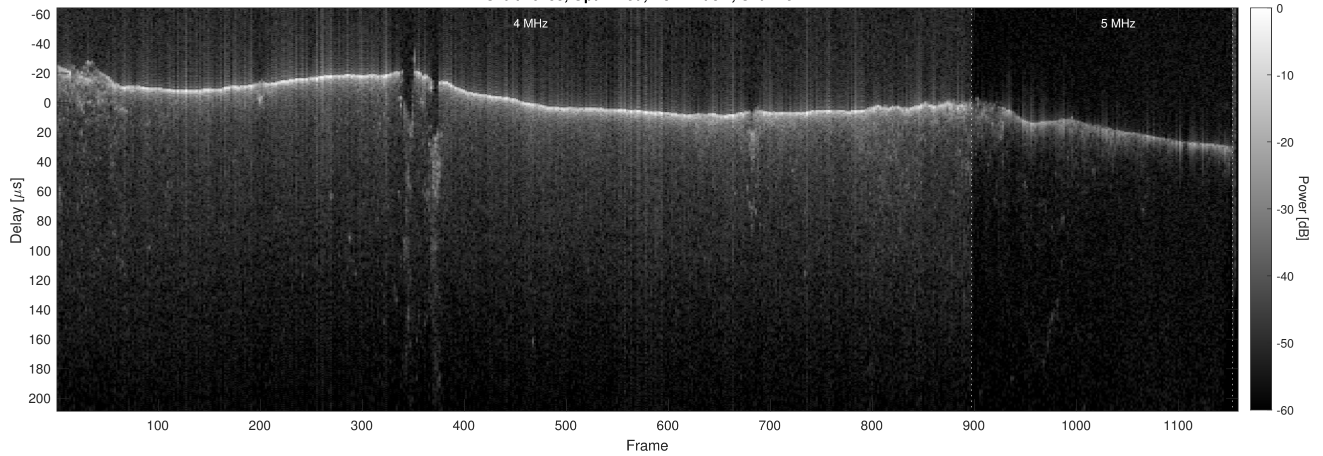
Orbit 10233, Optimized, No Window, Channel 2
