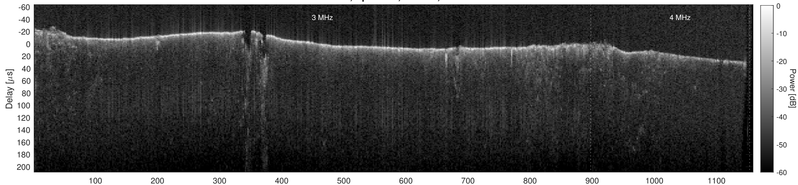
Orbit 10233, Cluttergram
