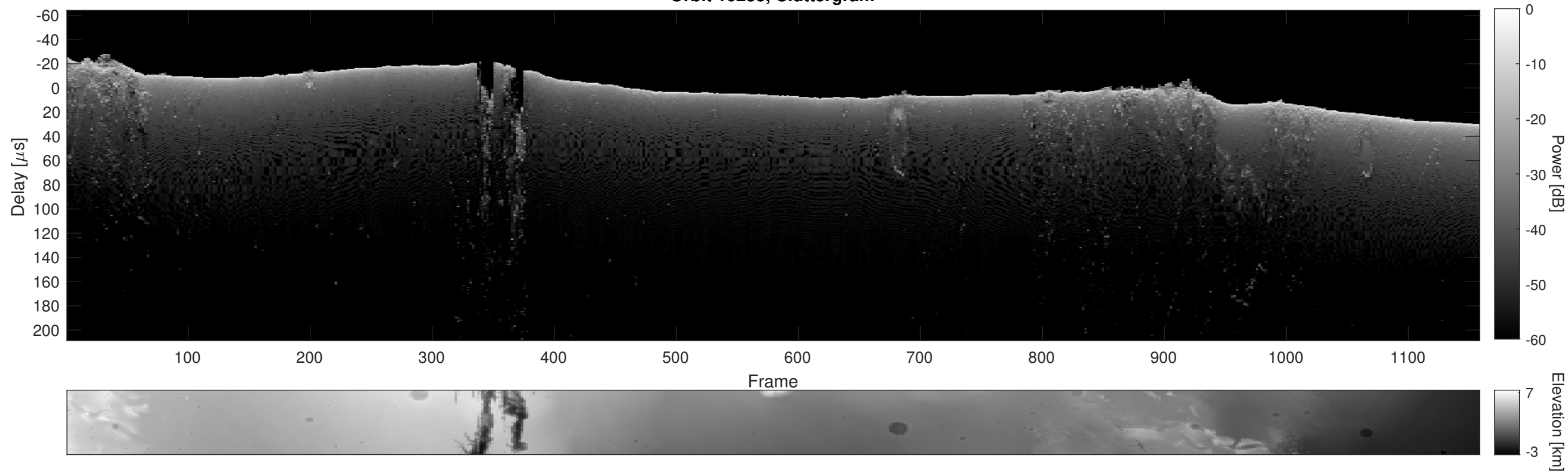
Orbit 10233, Cluttergram
