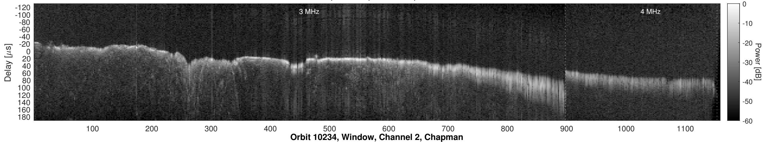
Orbit 10234, Window, Channel 2, Uncorrected
