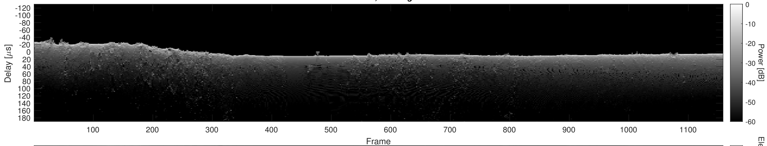
Orbit 10234, Cluttergram
