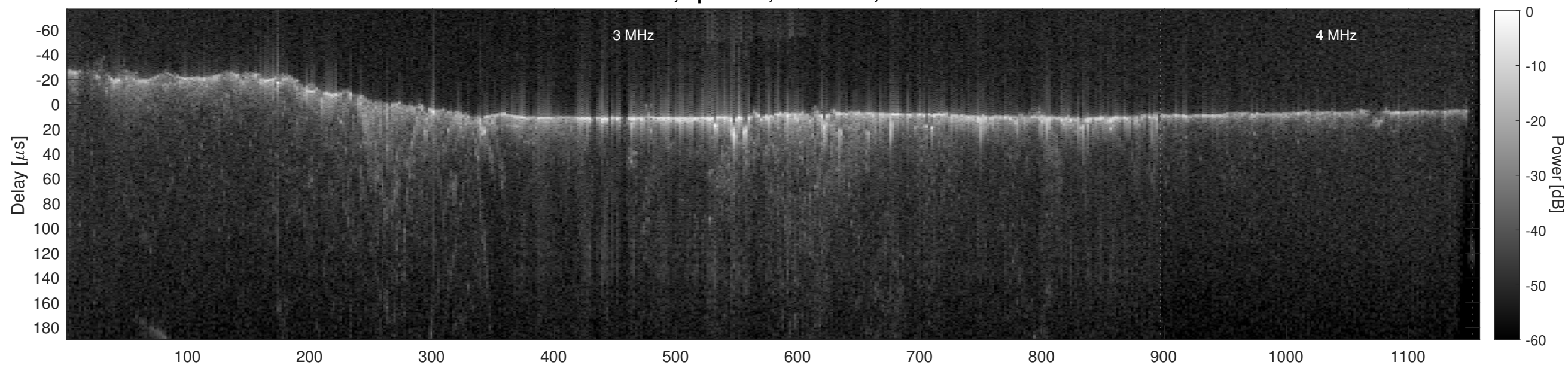
Orbit 10234, Cluttergram
