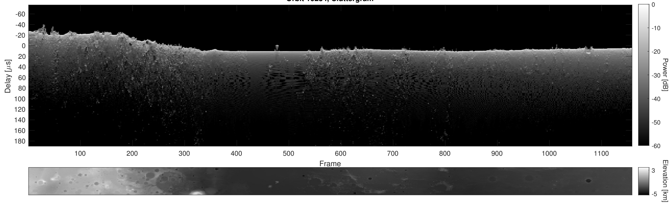
Orbit 10234, Cluttergram
