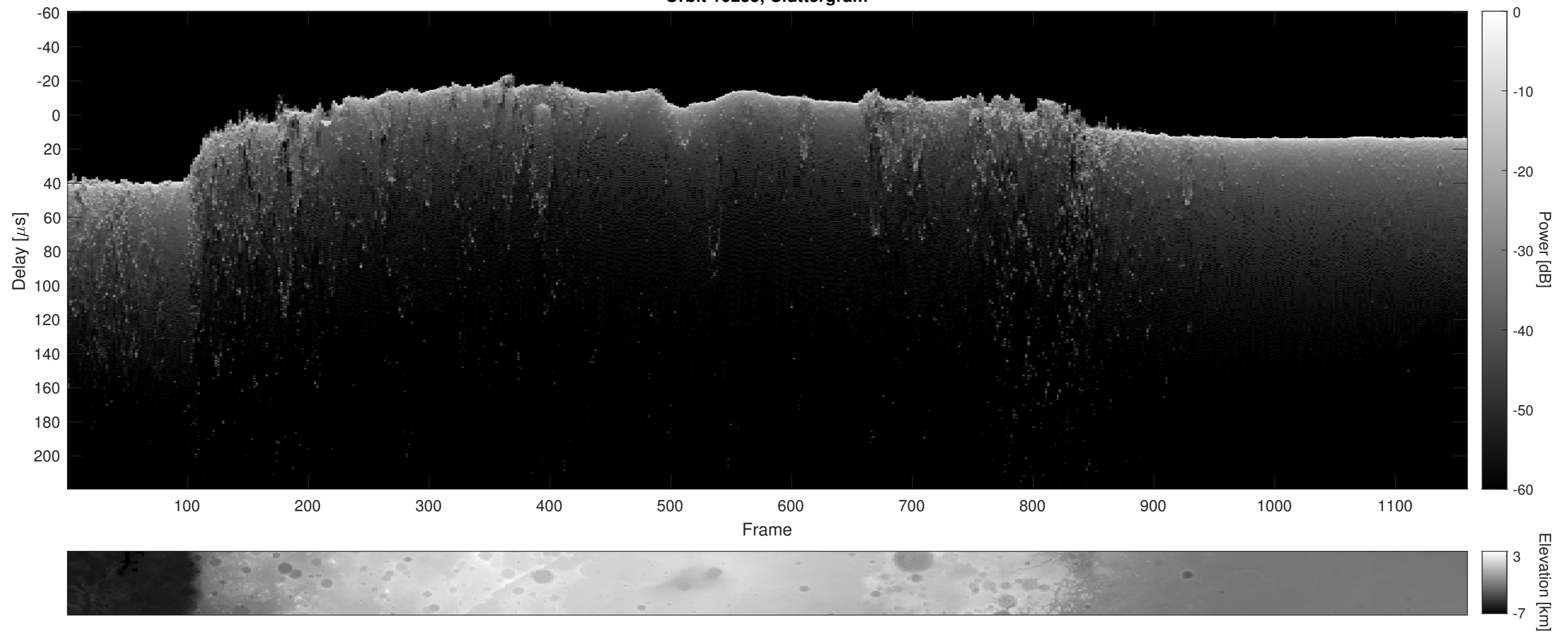
Orbit 10235, Cluttergram
