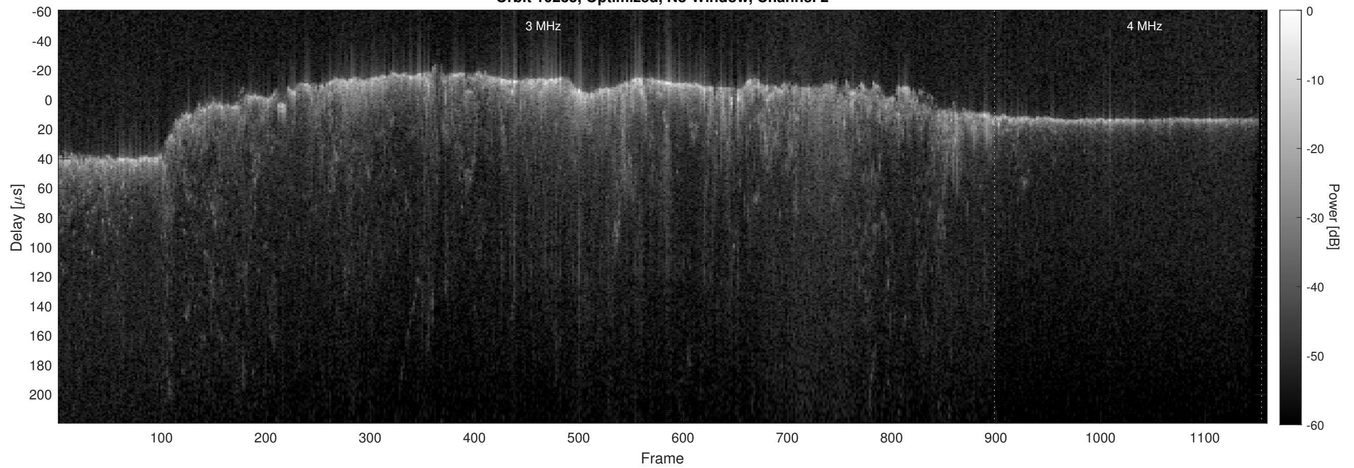
Orbit 10235, Optimized, No Window, Channel 2
