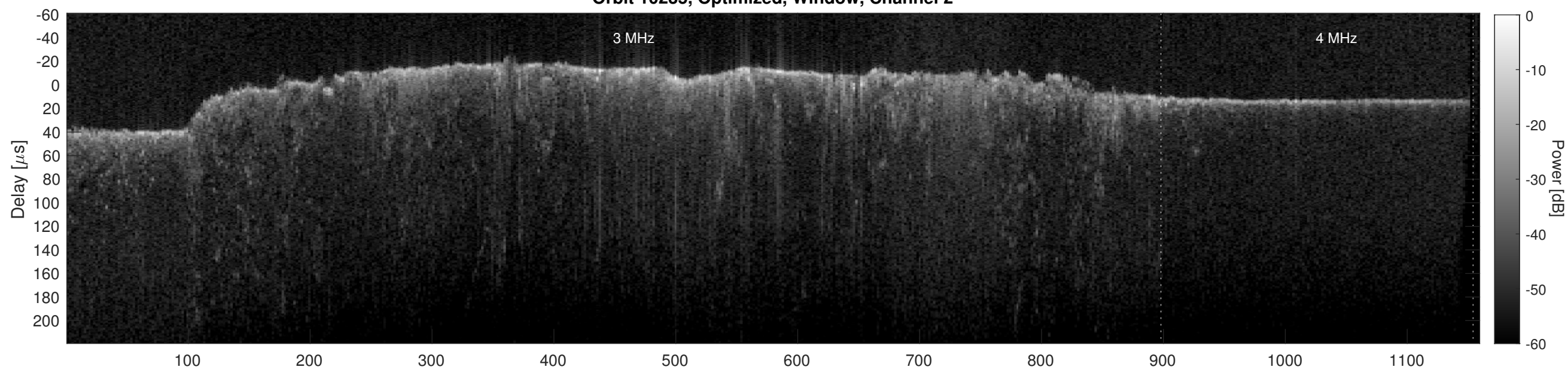
Orbit 10235, Cluttergram
