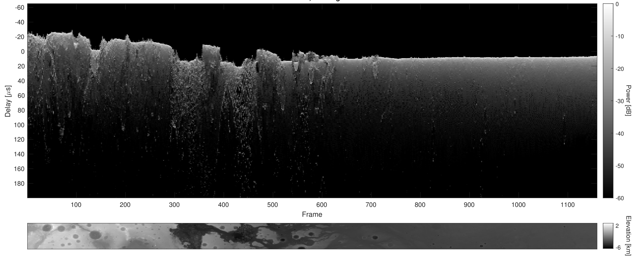
Orbit 10236, Cluttergram
