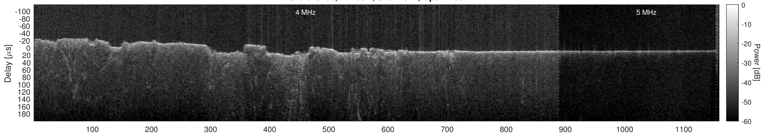
Orbit 10236, Cluttergram
