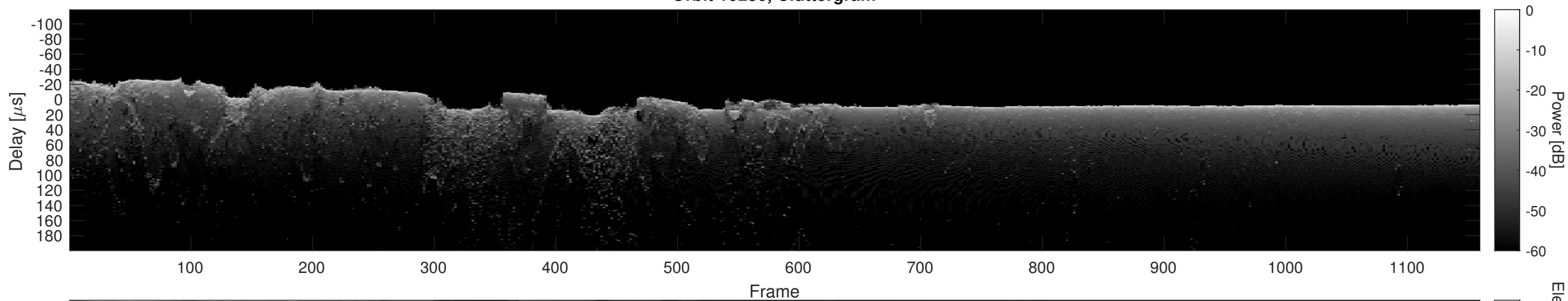
Orbit 10236, Cluttergram
