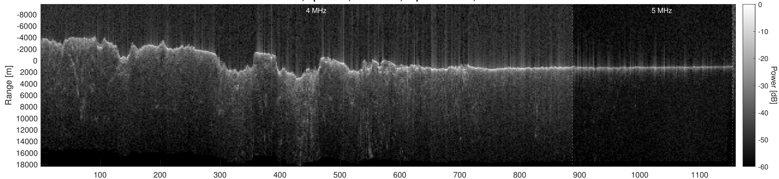
Orbit 10236, Optimized, No Window, Depth-Corrected, Channel 2
