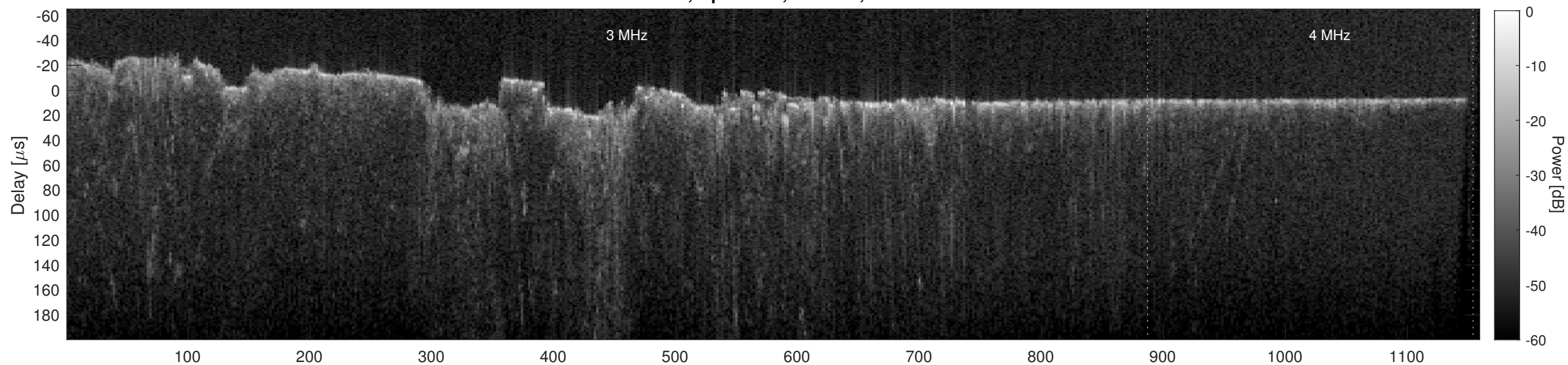
Orbit 10236, Cluttergram
