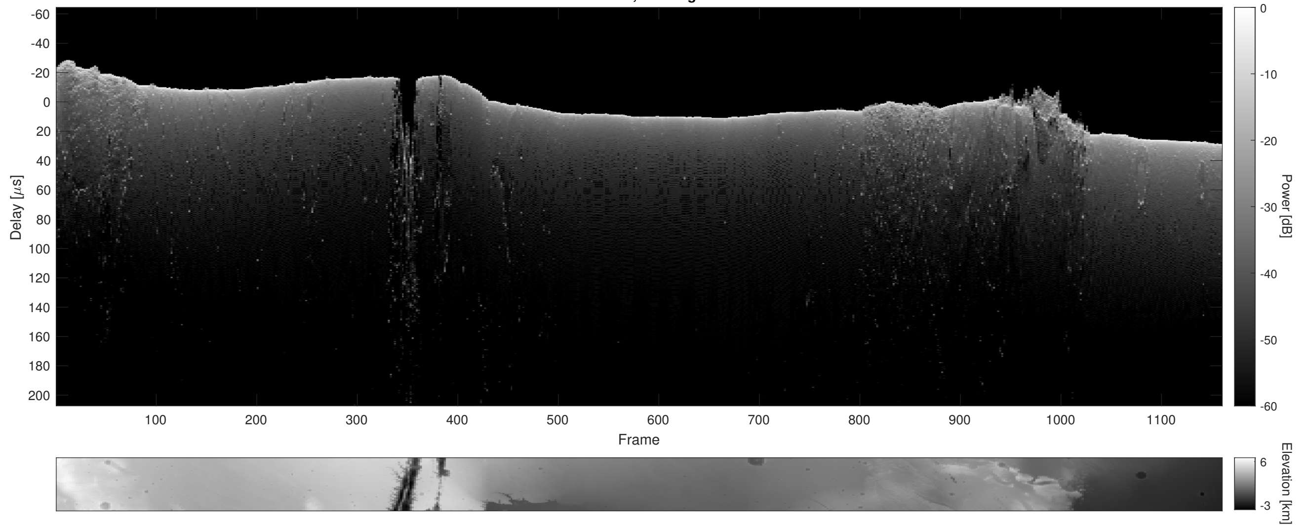
Orbit 10240, Cluttergram
