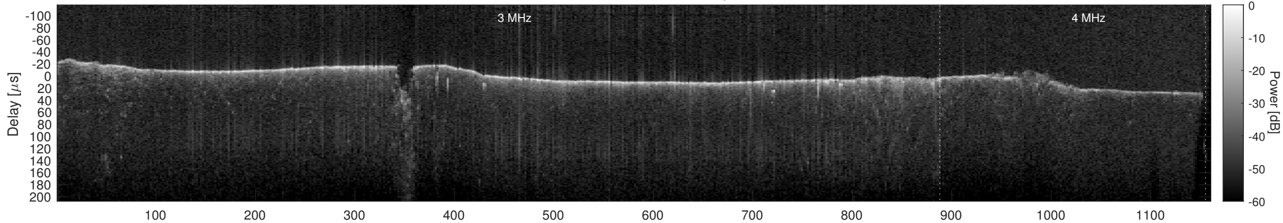
Orbit 10240, Cluttergram
