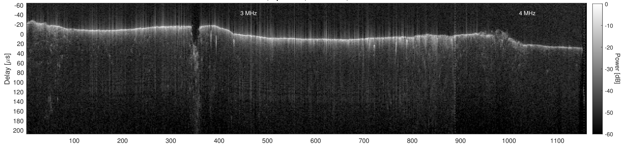
Orbit 10240, Cluttergram
