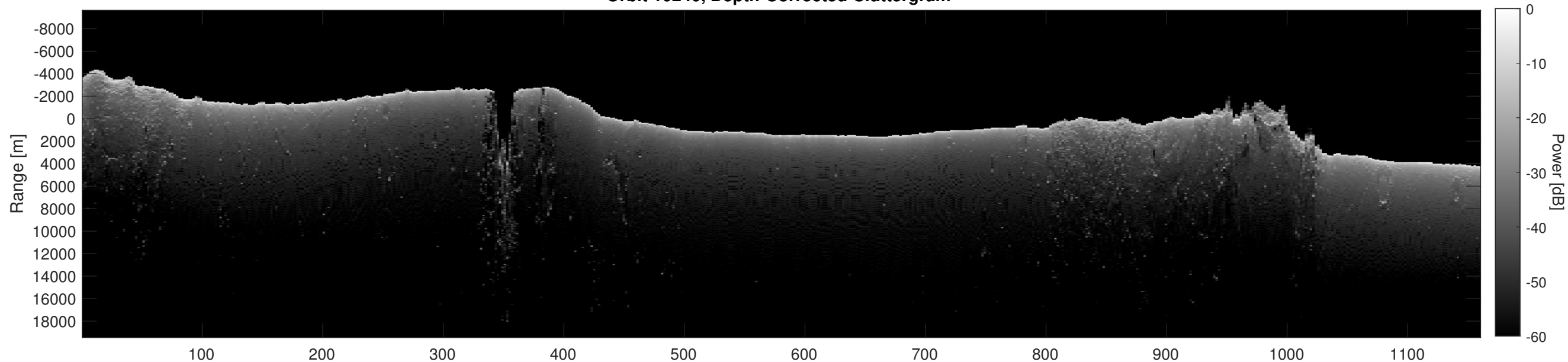
Orbit 10240, Depth-Corrected Cluttergram
