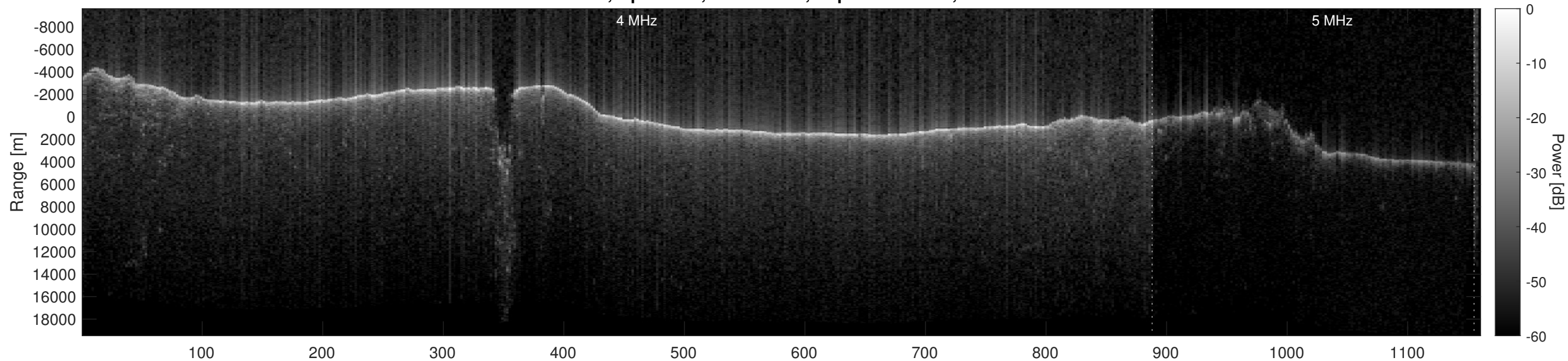
Orbit 10240, Optimized, No Window, Depth-Corrected, Channel 2
