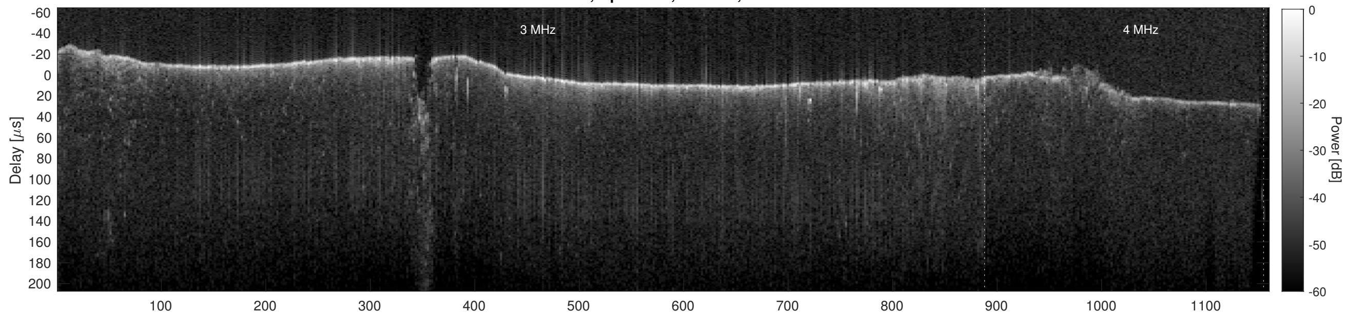
Orbit 10240, Cluttergram
