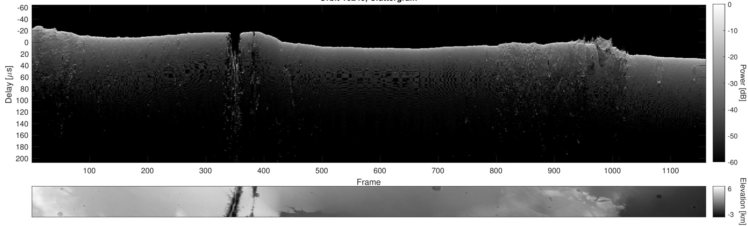
Orbit 10240, Cluttergram
