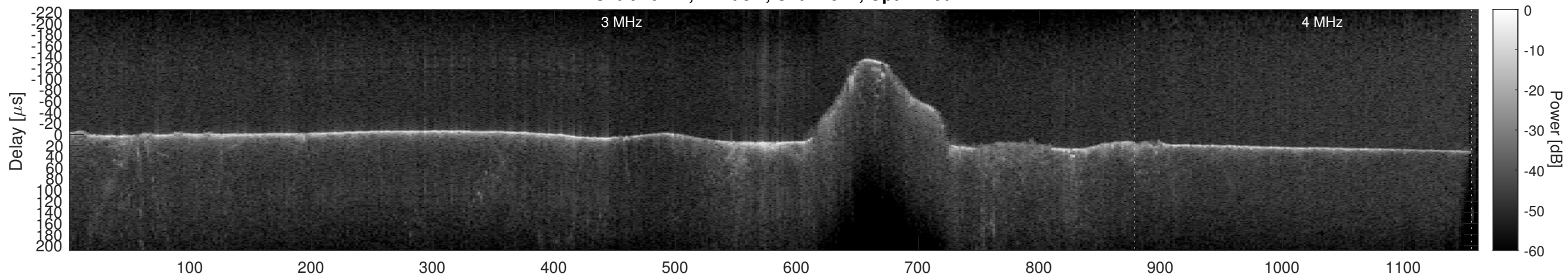
Orbit 10244, Cluttergram
