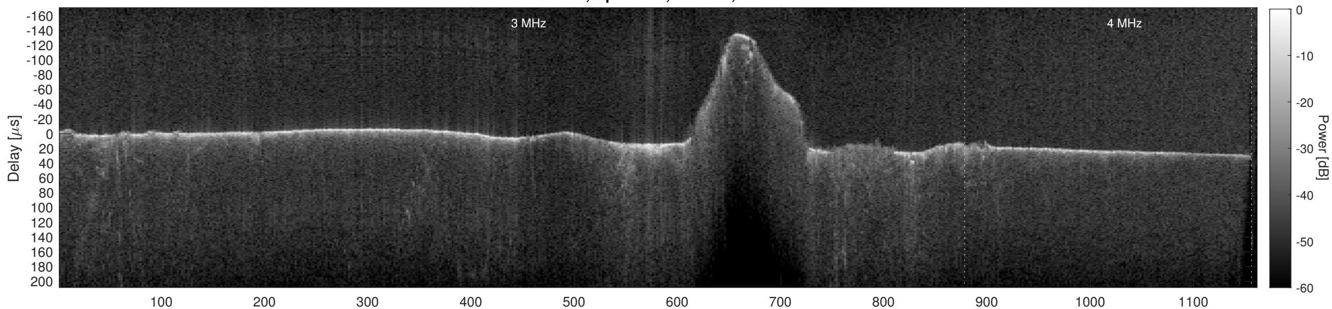
Orbit 10244, Cluttergram
