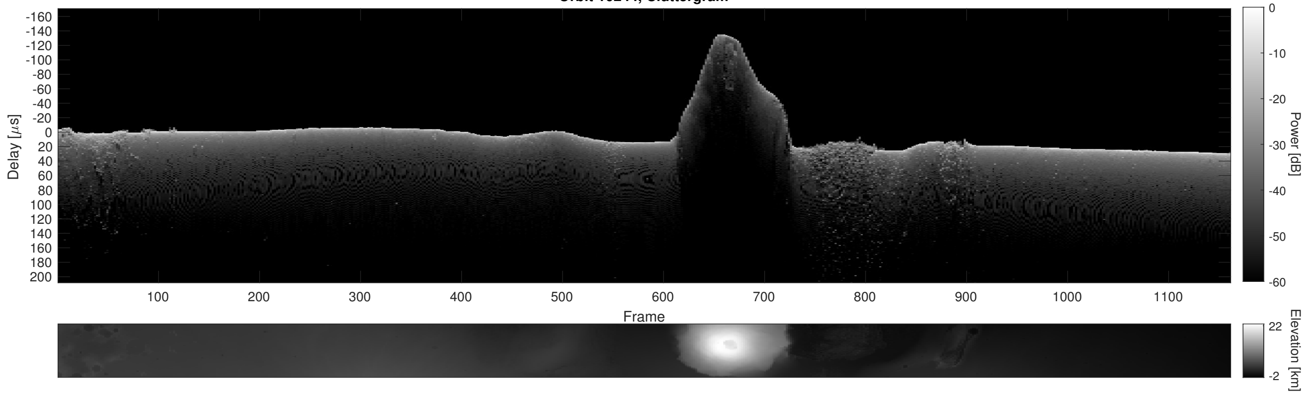
Orbit 10244, Cluttergram
