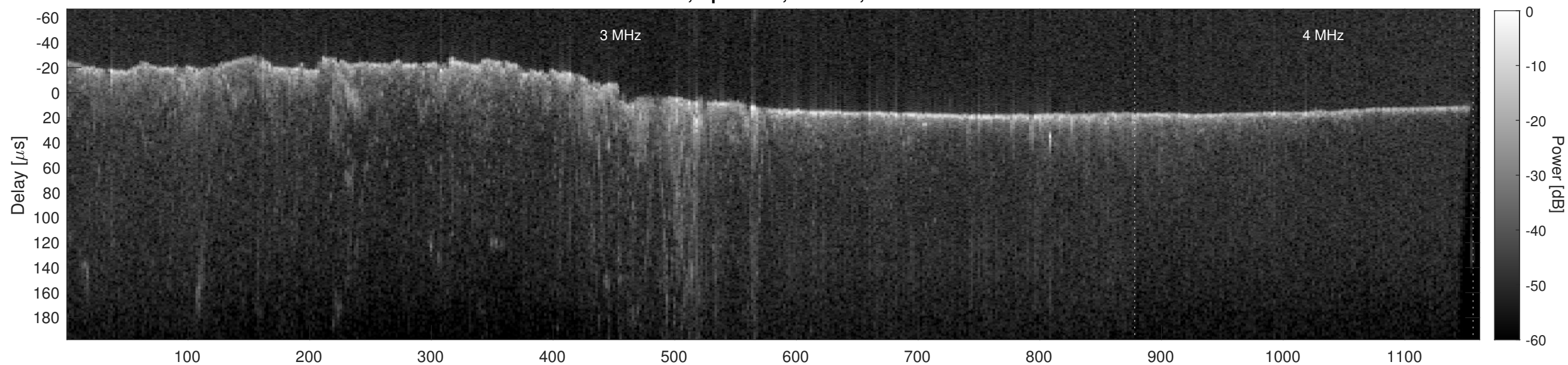
Orbit 10245, Cluttergram
