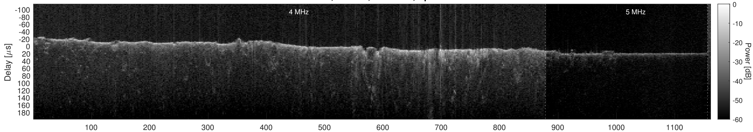
Orbit 10246, Cluttergram
