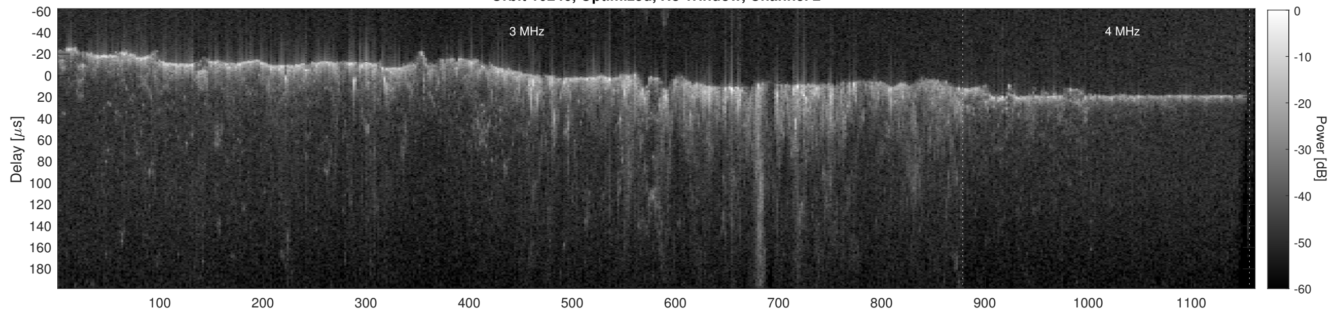
Orbit 10246, Cluttergram
