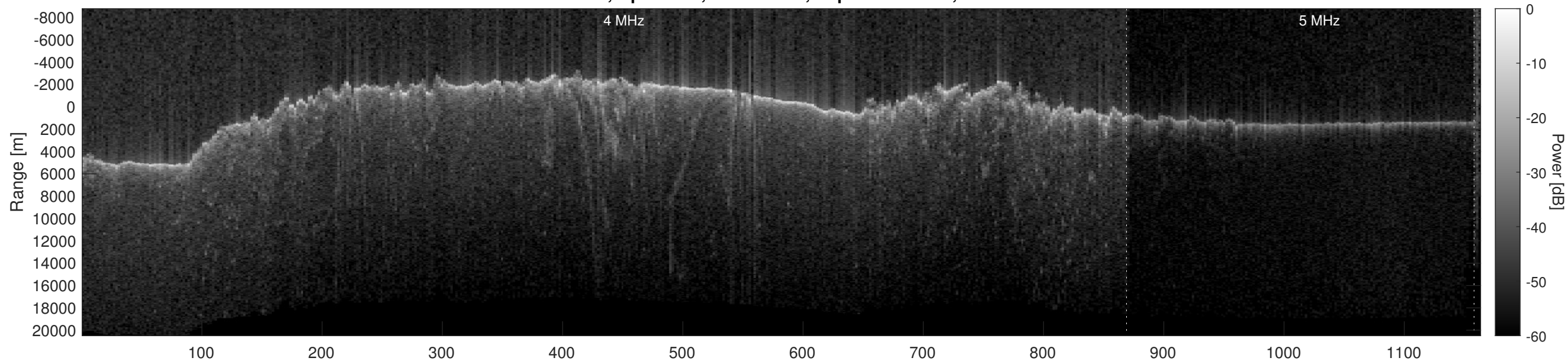
Orbit 10249, Optimized, No Window, Depth-Corrected, Channel 2
