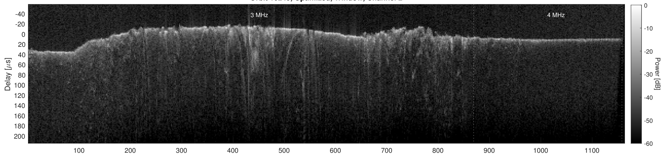
Orbit 10249, Cluttergram
