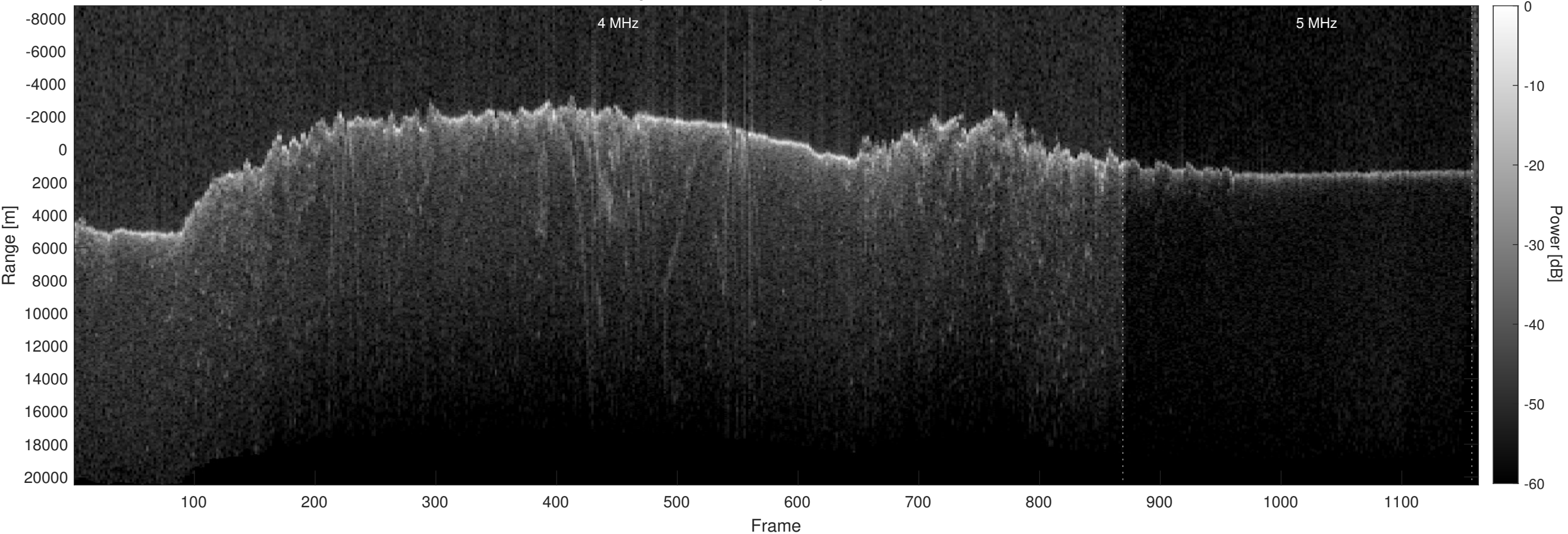
Orbit 10249, Optimized, Window, Depth-Corrected, Channel 2
