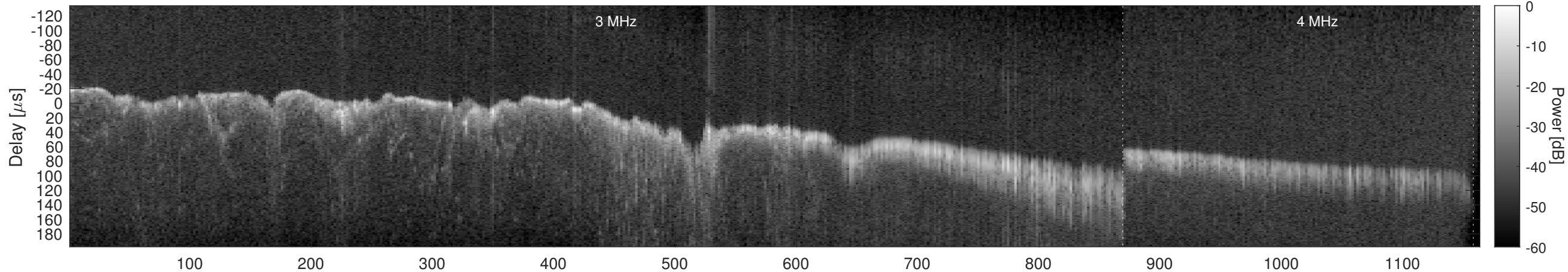
Orbit 10252, Window, Channel 2, Chapman
