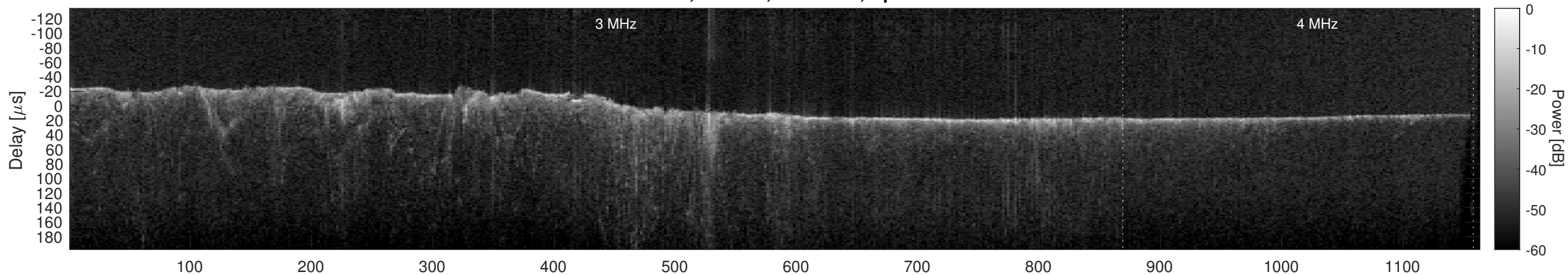
Orbit 10252, Cluttergram
