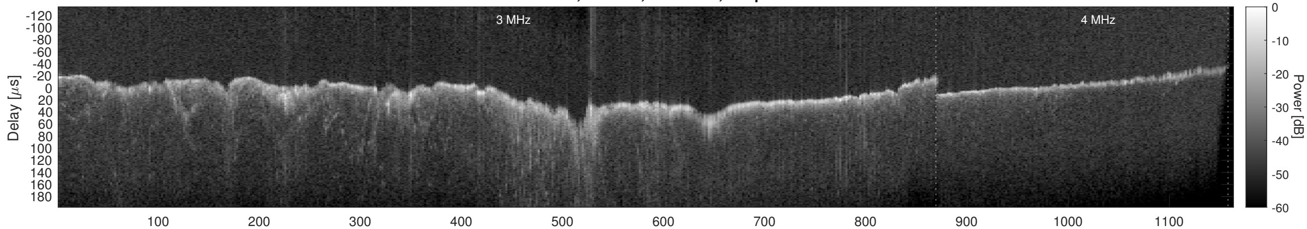
Orbit 10252, Window, Channel 2, Optimized
